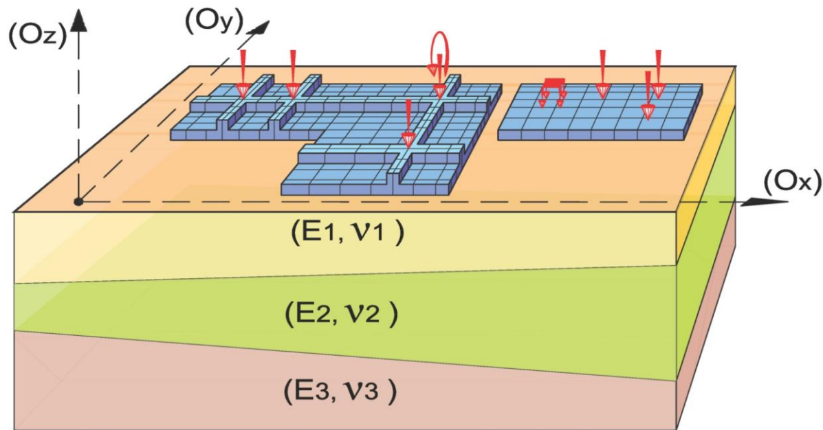
Rafts and slabs-on-grade
