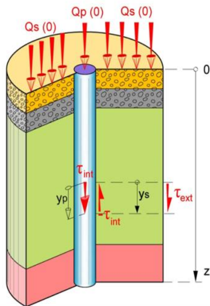
Piles under axial loading
