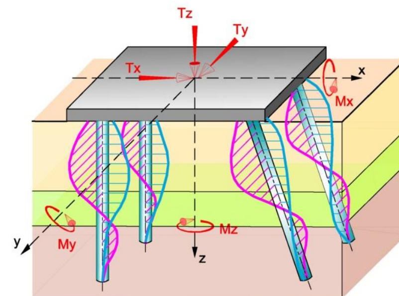
Pile group under combined loading
