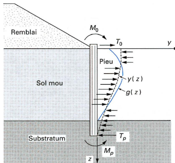
Downdrag and lateral soil pressures
