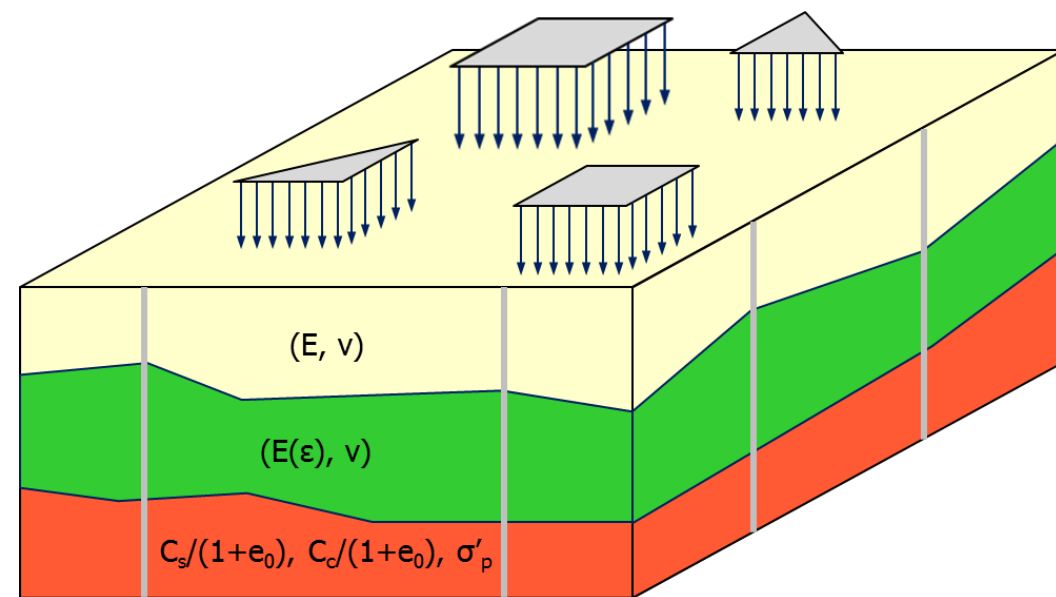
Embankments and flexible loads
