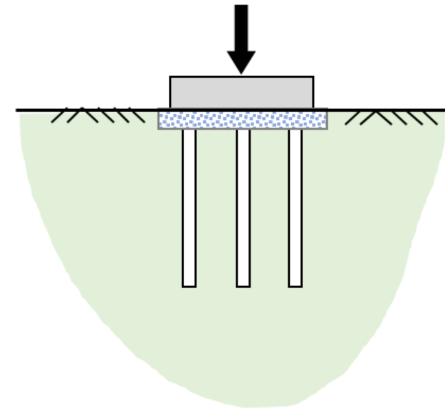
Footing on rigid inclusions
