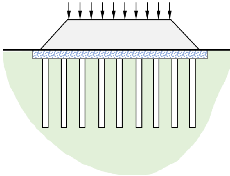
Embankment on rigid inclusions
