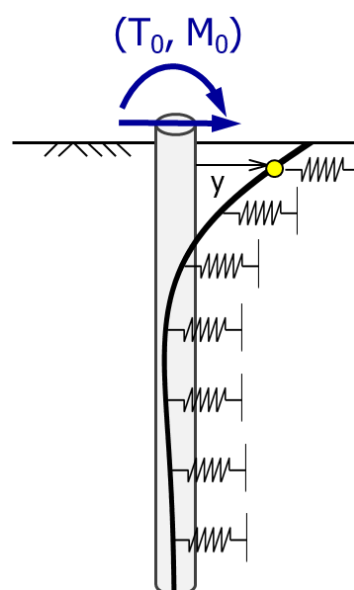
Piles under lateral loading
